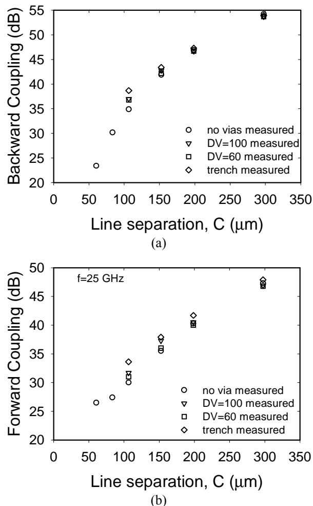
Figure 5: Measured (a) backward coupling and (b) forward coupling at 25 GHz of microstrip lines fabricated on different layers of polyimide (Figure 1b) as a function of center to center spacing, C.
